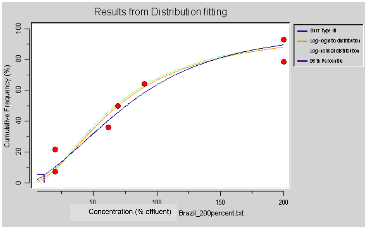
Figure 2: BurrliOZ distribution for Brazilian effluent results if >100% is taken to be 200% (using an ACR of 10 for acute studies). There were seven data points in this distribution, from five different taxonomic groups. Note that the software advises caution in interpretation of results with less than eight species. Burr Type III distribution: Trigger value for 95% protection level = 11% effluent Trigger value for 99% protection level = 3% effluent Log-logistic distribution: Trigger value for 95% protection level = 13% effluent Trigger value for 99% protection level = 6% effluent
