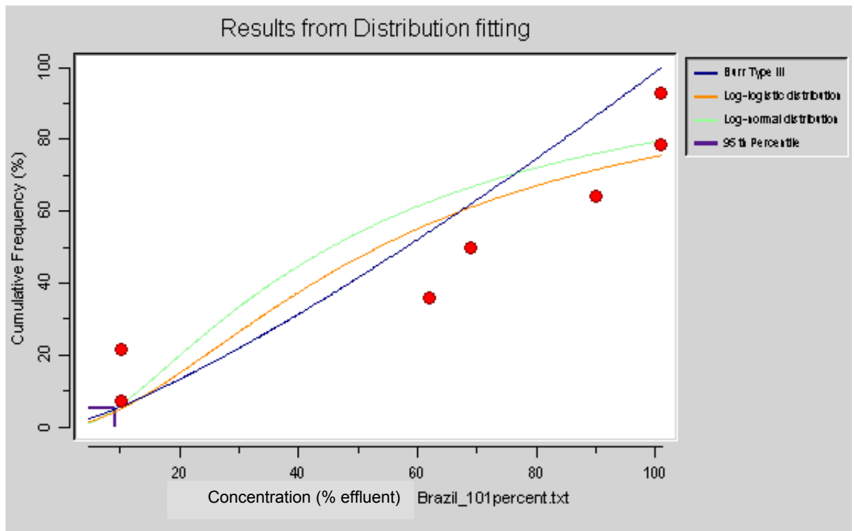
Figure 1: BurrliOZ distribution for Brazilian effluent results if >100% is taken to be 101% (using an ACR of 10 for acute studies). There were seven data points in this distribution, from five different taxonomic groups. Note that the software advises caution in interpretation of results with less than eight species. Burr Type III distribution: Trigger value for 95% protection level = 9% effluent Trigger value for 99% protection level = 3% effluent Log-logistic distribution: Trigger value for 95% protection level = 11% effluent Trigger value for 99% protection level = 5% effluent
